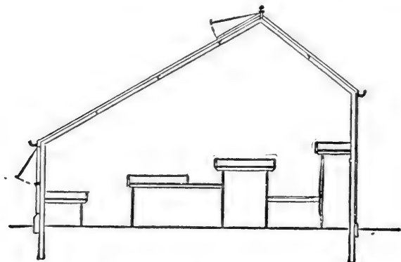
FIG. 80. SECTION OF IRON ROSE HOUSE.
